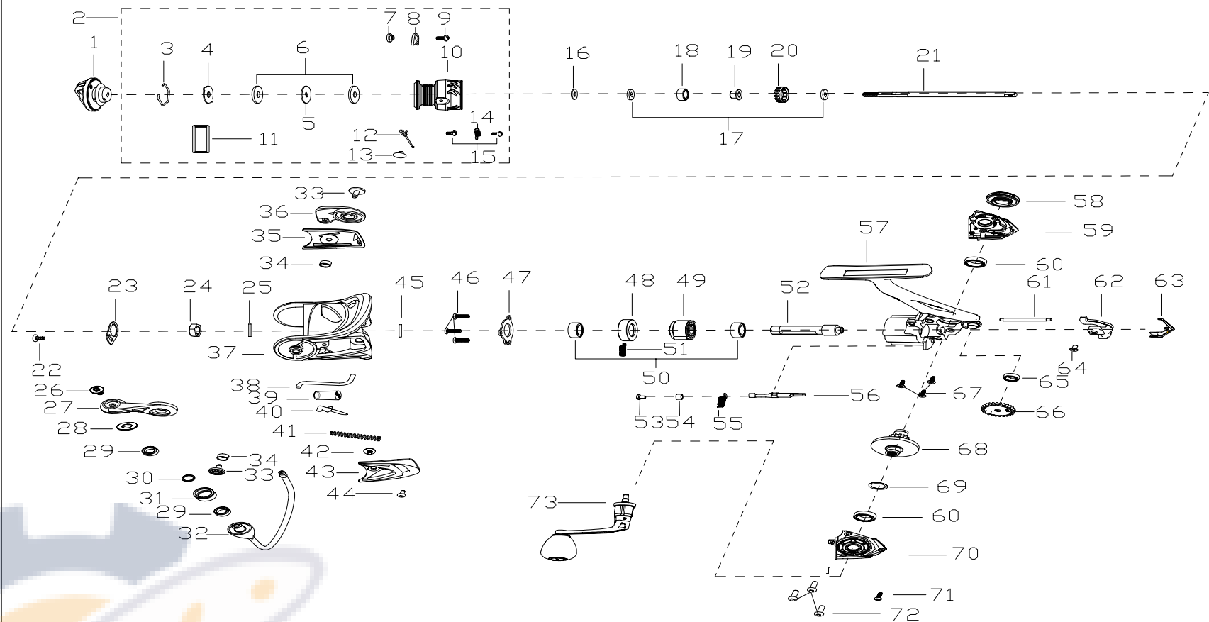
PARTS LIST OF CS7-1000
